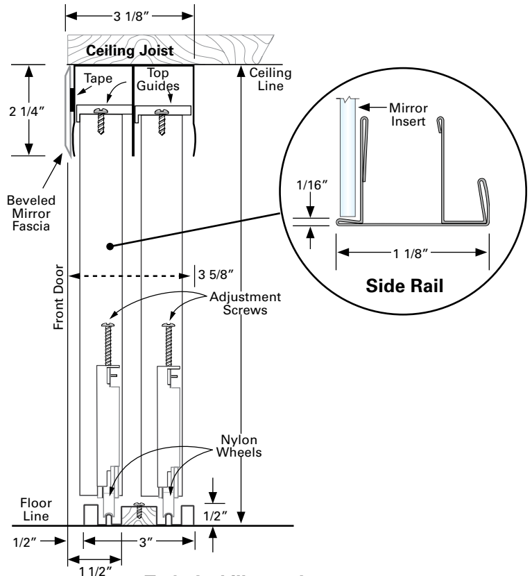
Technical Illustration
