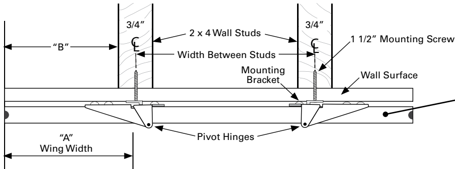
Technical Illustration
