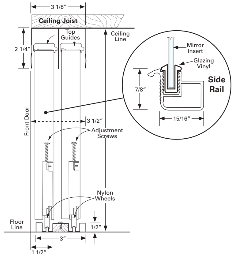
Technical Illustration
